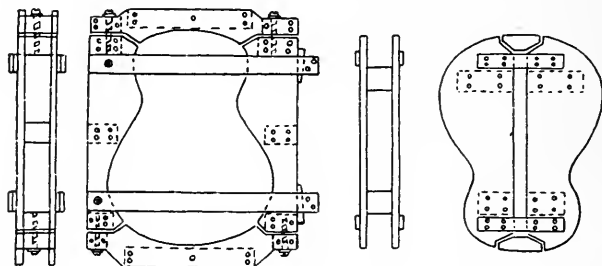
FIG. 409. FORM AND FOLLOW BOARDS IN CAUL WORK.
